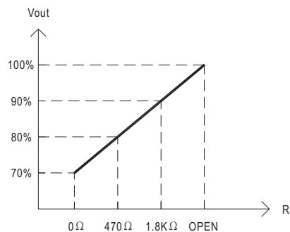
Fig. 2.2 External Resistance (Typical)
