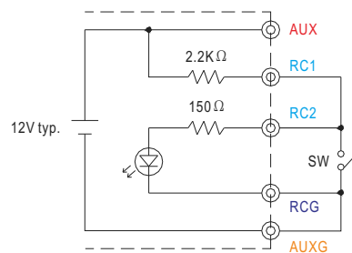
Example 3.2(C): Using internal 12V auxiliary output
