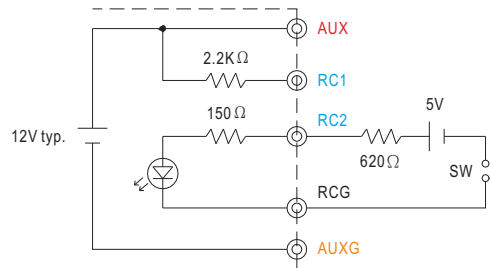
Example 3.2(B): Using internal 12V auxiliary output
